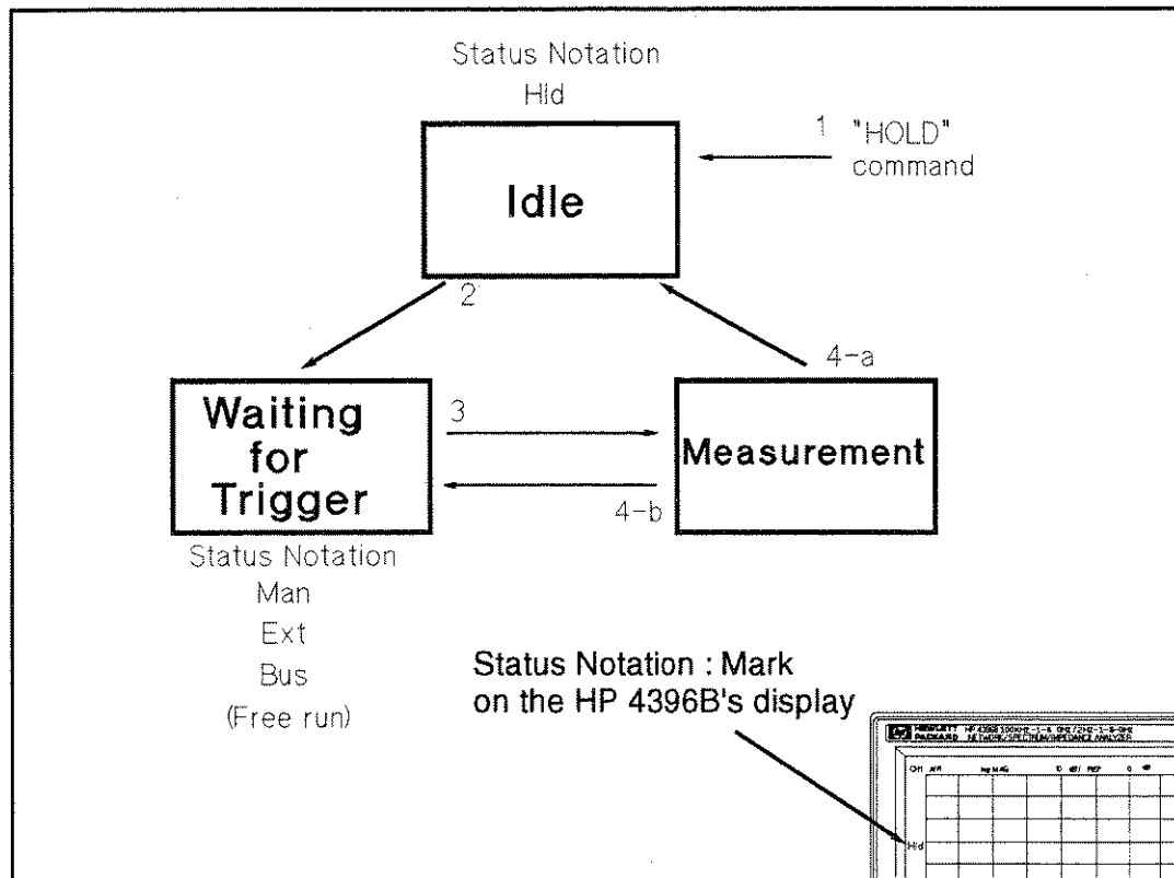
Figure 2-1. Trigger System
