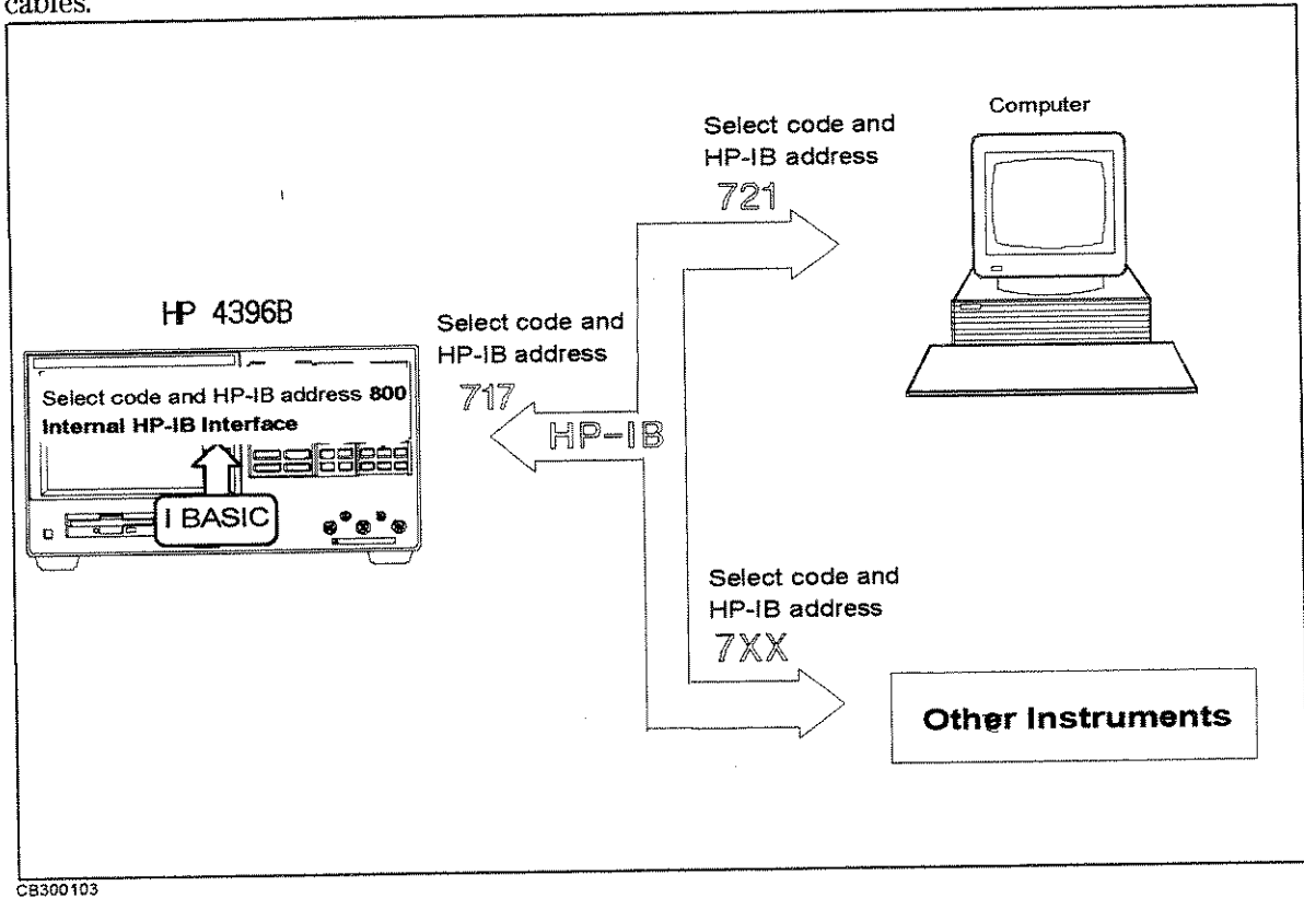
Figure 1-1. System Configuration for HP-IB Remote Control
