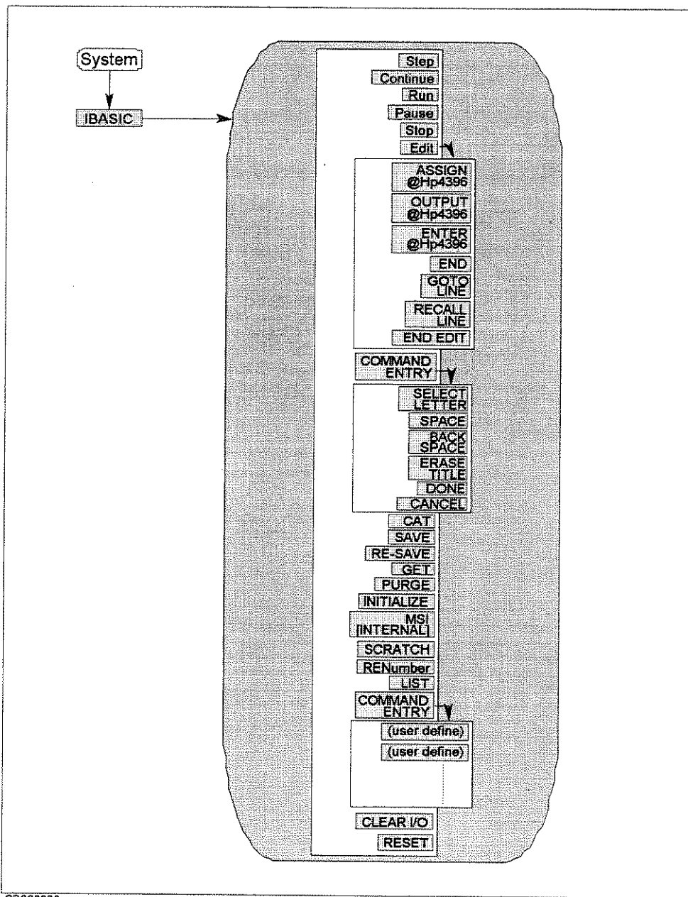
Figure D-1. IBASIC Menu
