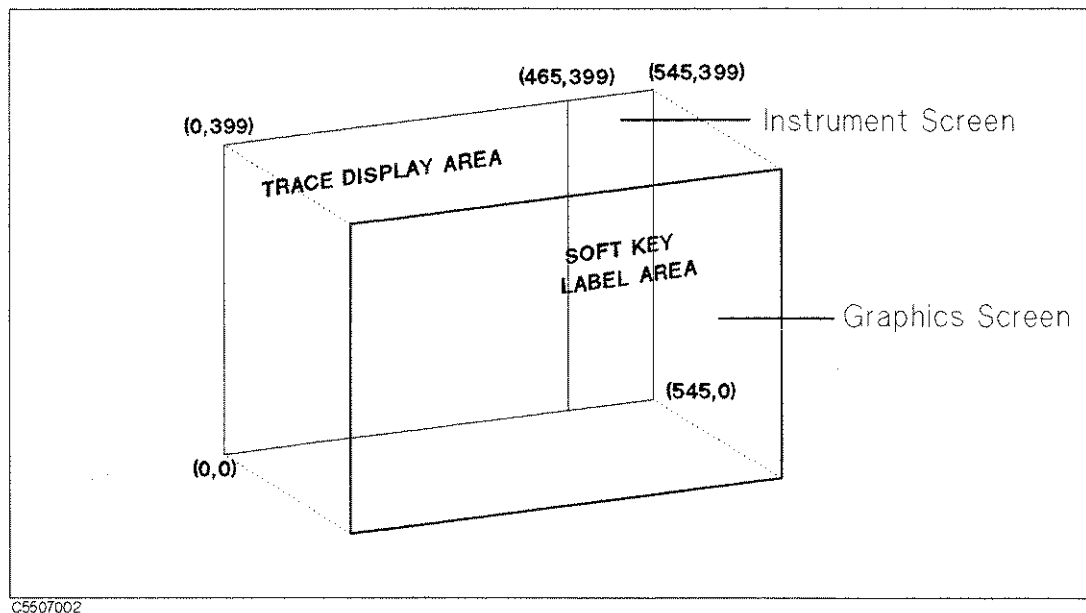
Figure 7-1. Screen Structure
