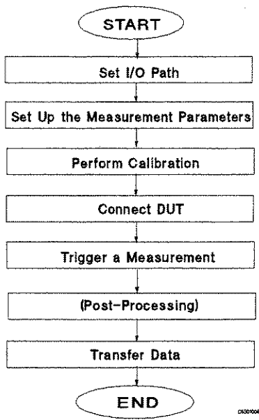
Figure 1-2. Program Flow
